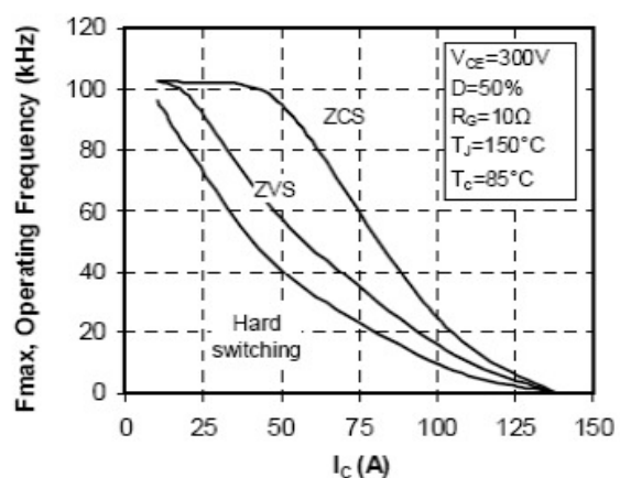
Fig 6. Operating Frequency vs. Collector Current
