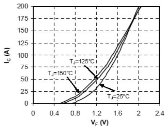
Fig 5. Forward Characteristics of Diode
