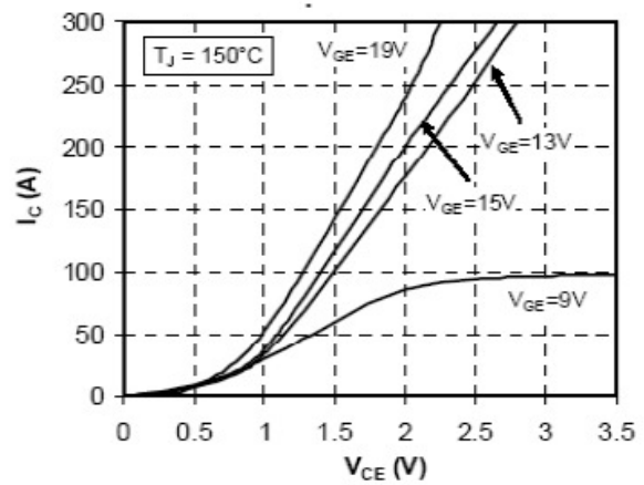
Fig 2. Typ. IGBT Output Characteristics
