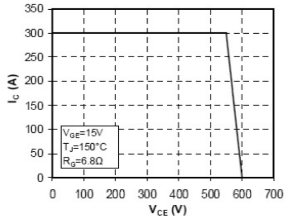
Fig 4. Reverse Bias Safe Operation Area
