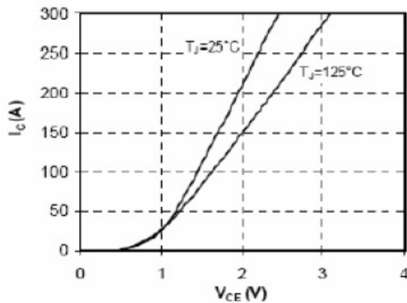
Fig 1. Typ. IGBT Output Characteristics
