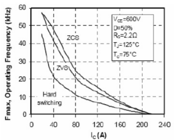
Fig 6. Operating Frequency vs. Collector Current
