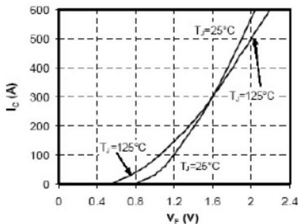
Fig 5. Forward Characteristics of Diode
