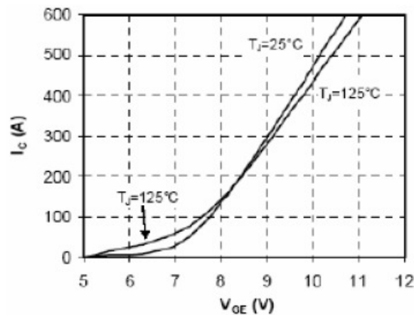
Fig 3. Typ. Transfer Characteristics
