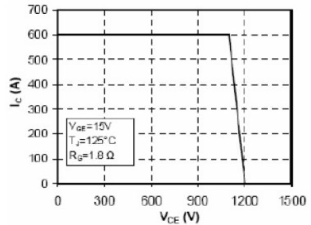
Fig 4. Reverse Bias Safe Operation Area
