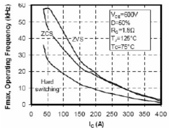
Fig 6. Operating Frequency vs. Collector Current
