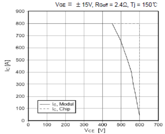
Fig 4. Reverse Bias Safe Operation Area
