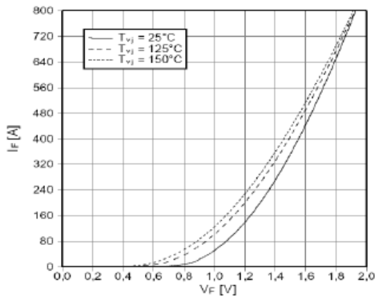
Fig 5. Forward Characteristics of Diode
