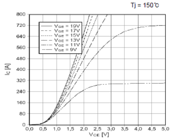
Fig 2. Typ. IGBT Output Characteristics
