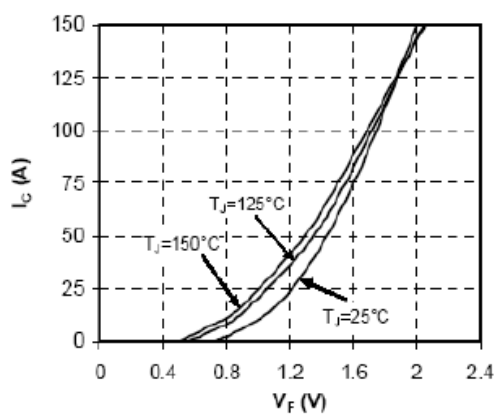
Fig 5. Forward Characteristics of Diode
