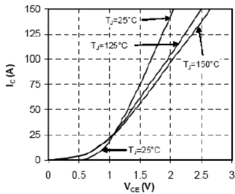
Fig 1. Typ. IGBT Output Characteristics
