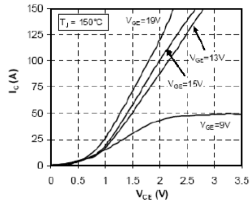
Fig 2. Typ. IGBT Output Characteristics
