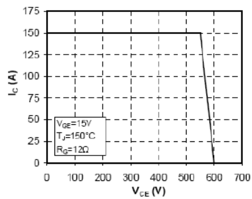
Fig 4. Reverse Bias Safe Operation Area
